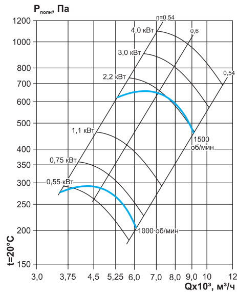
ВКР №5,0 (D=d1,0)
