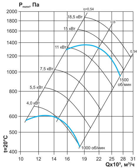
ВКР №8,0 (D=d0,9)
